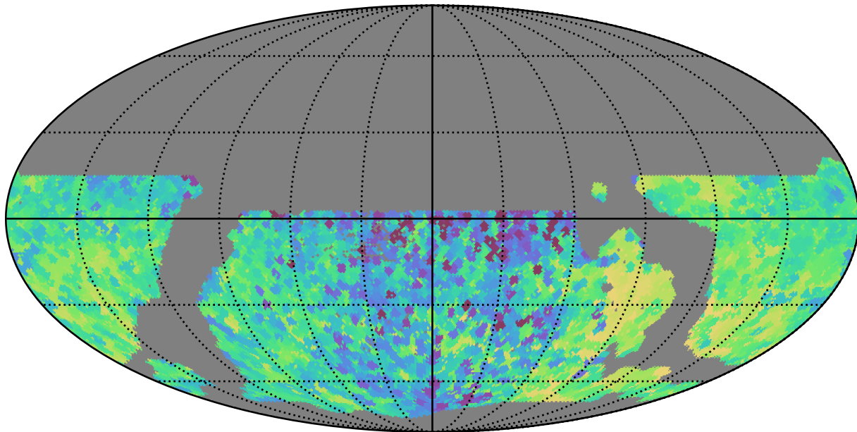
weather_cloudso30v3.4_10yrs WFD y band: Min skyBrightness
