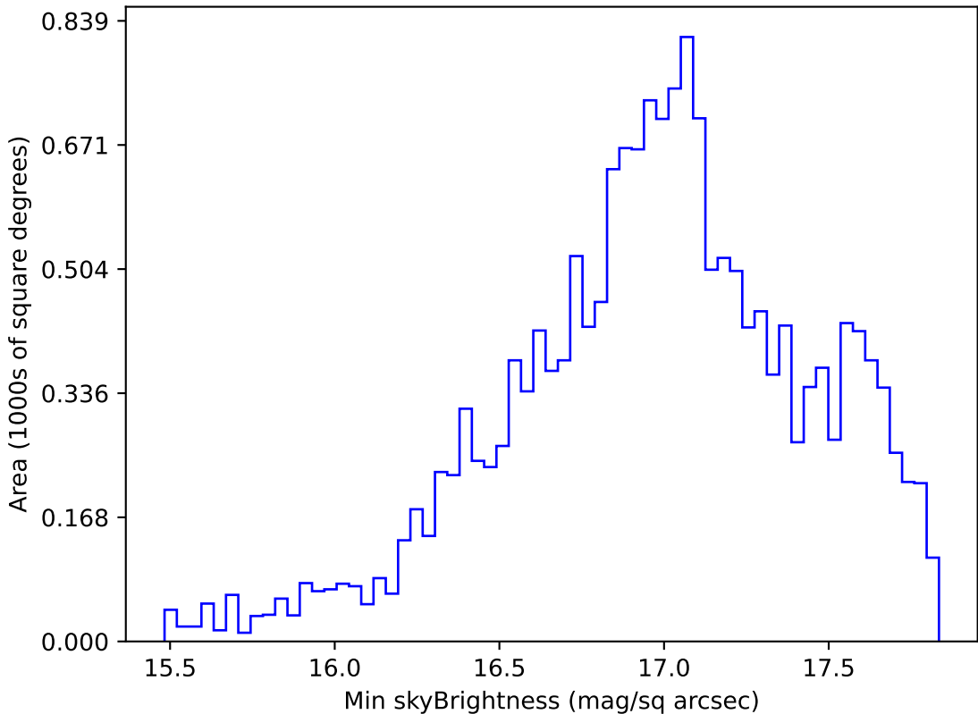
weather_cloudso30v3.4_10yrs WFD y band: Min skyBrightness
