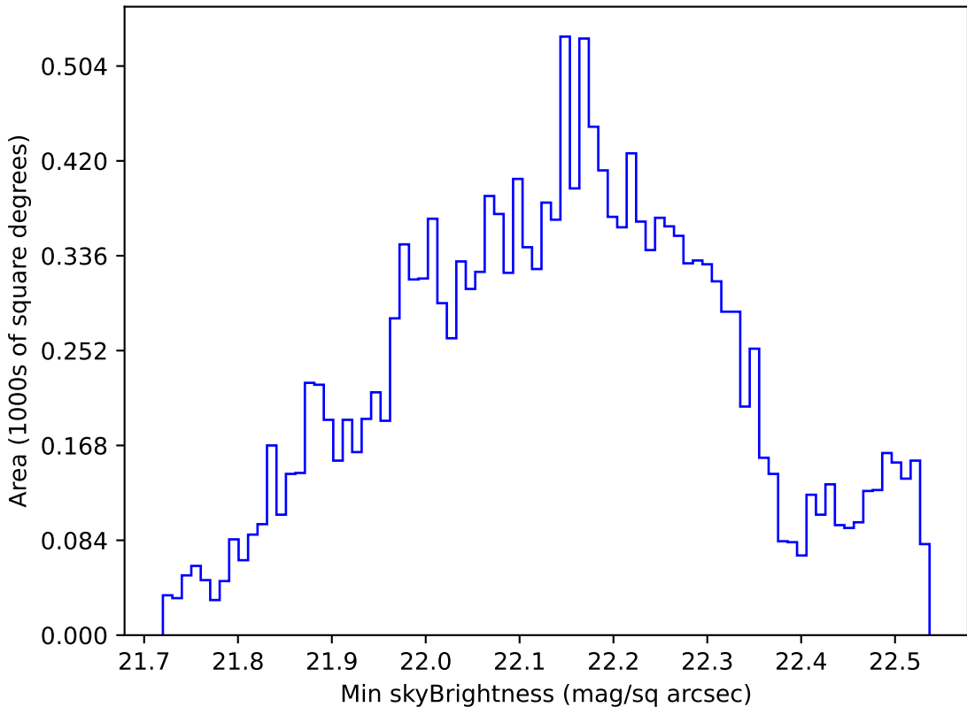
weather_cloudso30v3.4_10yrs WFD u band: Min skyBrightness
