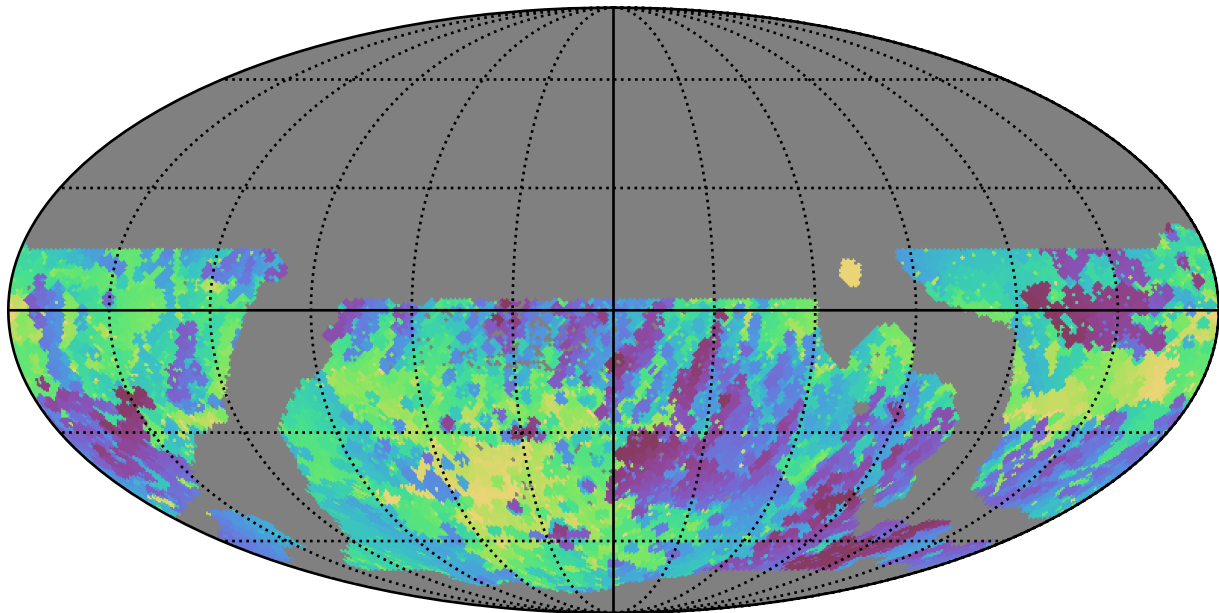
weather_cloudso30v3.4_10yrs WFD r band: Min skyBrightness
