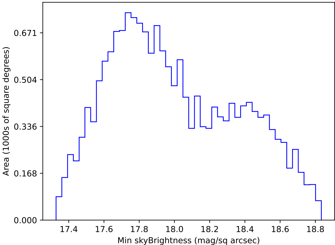
weather_cloudso30v3.4_10yrs WFD i band: Min skyBrightness
