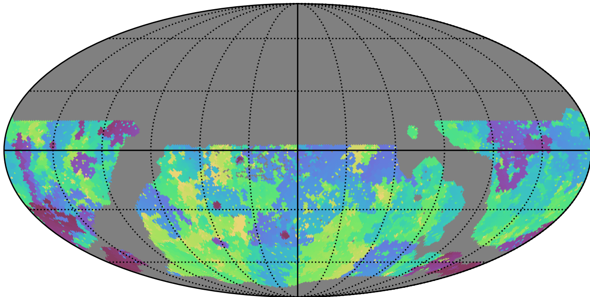
weather_cloudso30v3.4_10yrs WFD g band: Min skyBrightness
