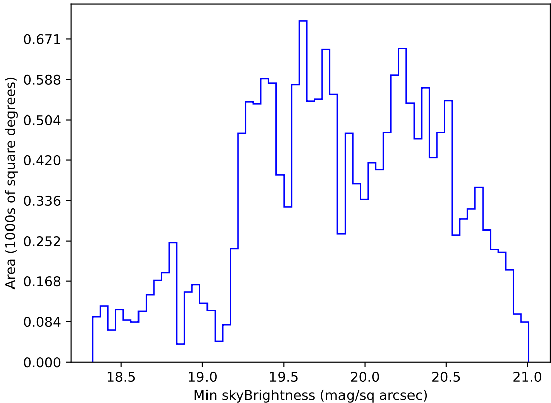
weather_cloudso30v3.4_10yrs WFD g band: Min skyBrightness
