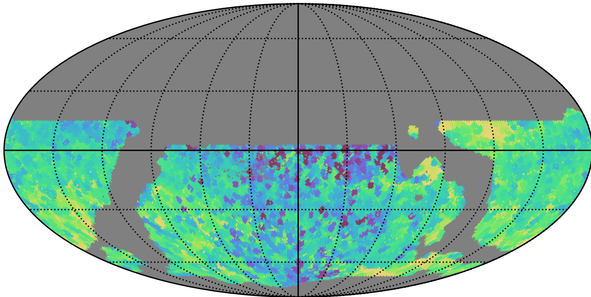
weather_cloudso30v3.4_10yrs WFD all bands: Min skyBrightness
