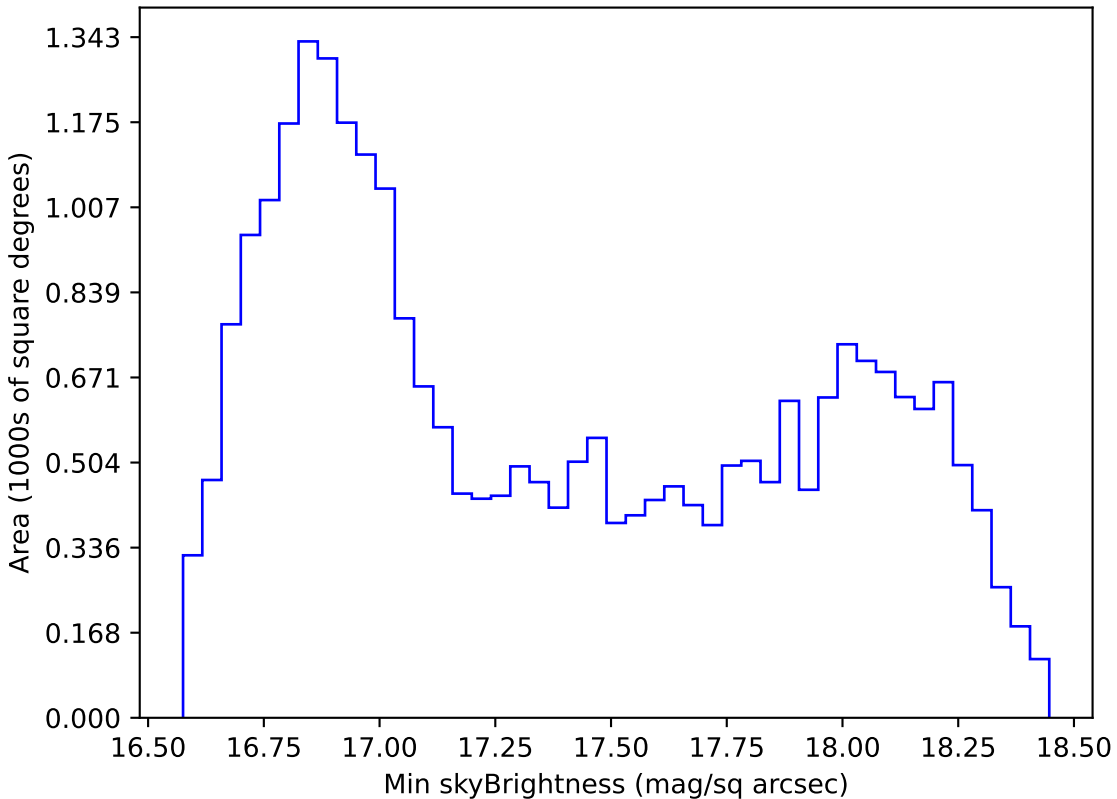
weather_cloudso30v3.4_10yrs All sky z band: Min skyBrightness
