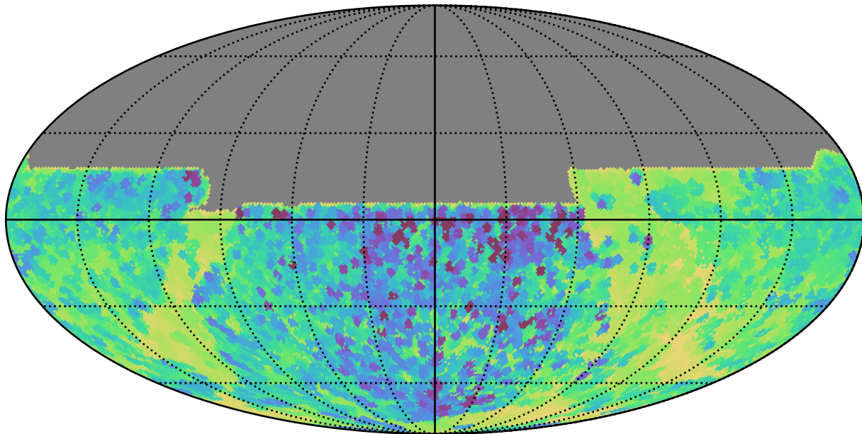
weather_cloudso30v3.4_10yrs All sky y band: Min skyBrightness
