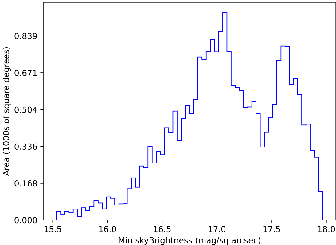
weather_cloudso30v3.4_10yrs All sky y band: Min skyBrightness
