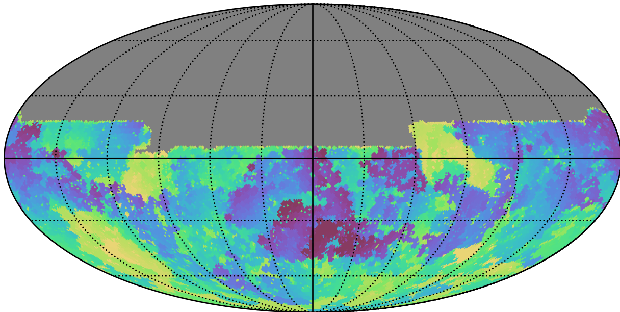
weather_cloudso30v3.4_10yrs All sky u band: Min skyBrightness
