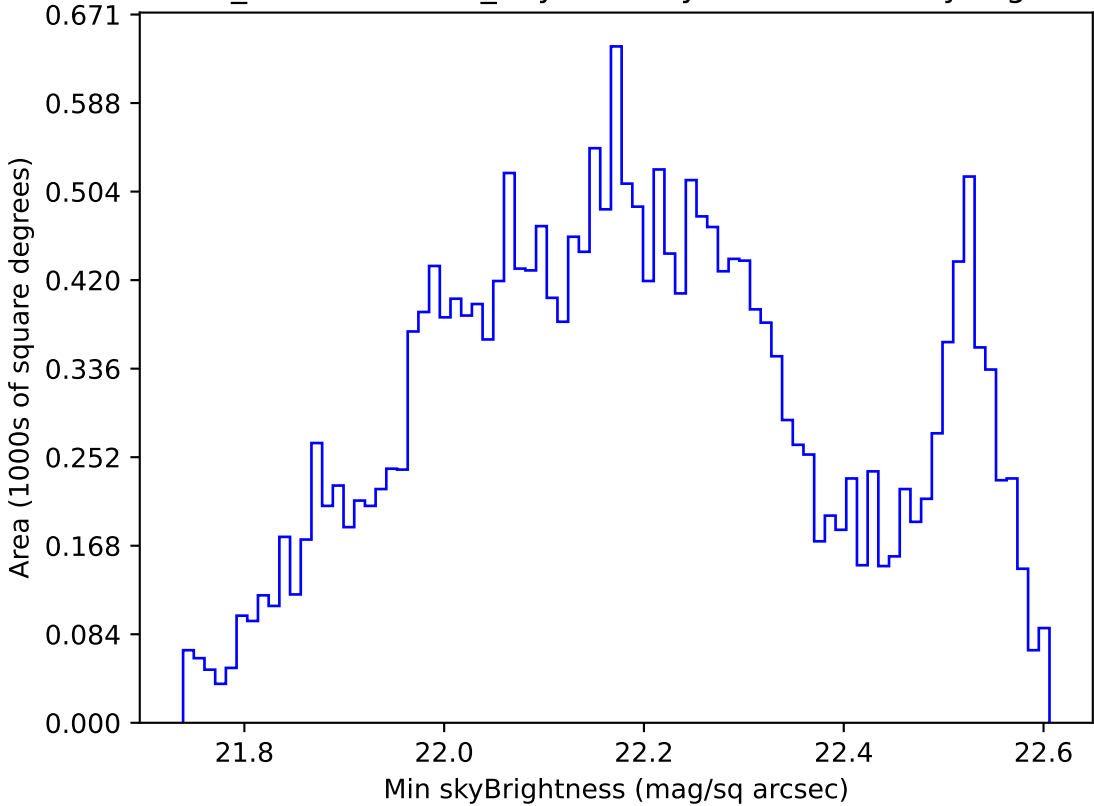
weather_cloudso30v3.4_10yrs All sky u band: Min skyBrightness
