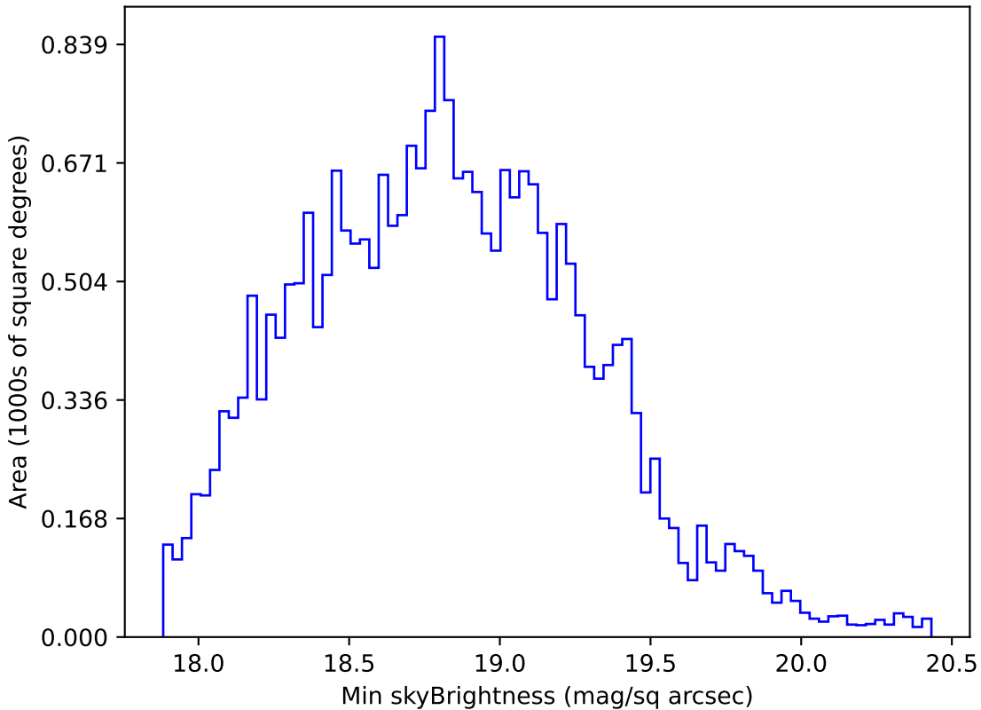
weather_cloudso30v3.4_10yrs All sky r band: Min skyBrightness
