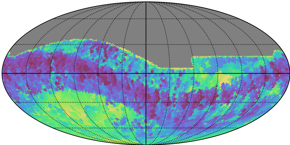
weather_cloudso30v3.4_10yrs All sky i band: Min skyBrightness
