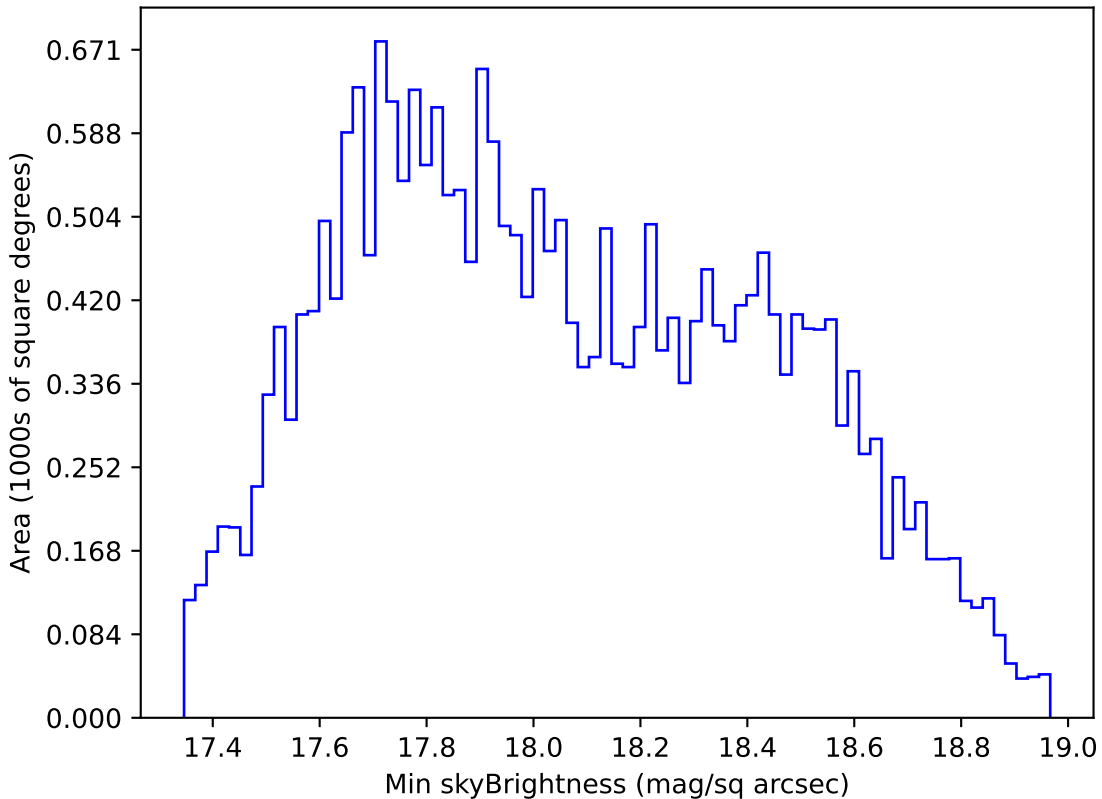
weather_cloudso30v3.4_10yrs All sky i band: Min skyBrightness
