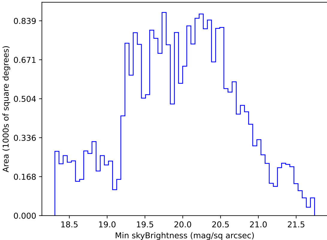
weather_cloudso30v3.4_10yrs All sky g band: Min skyBrightness
