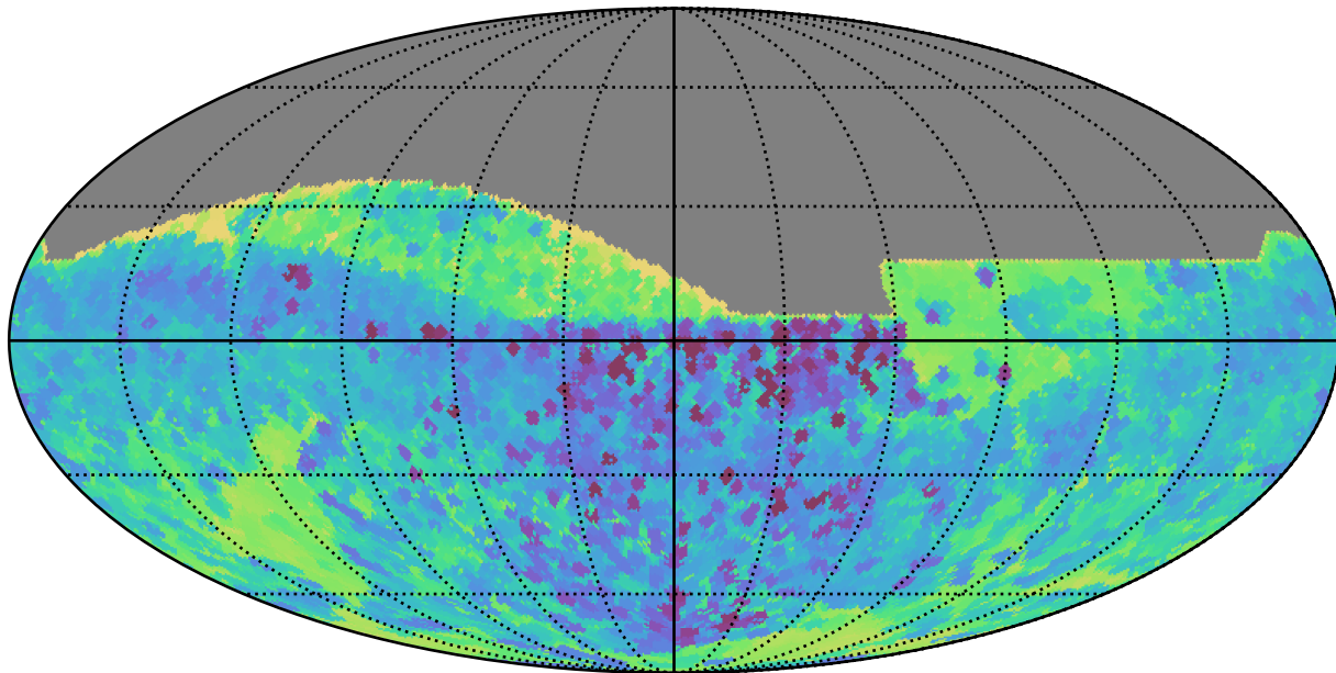
weather_cloudso30v3.4_10yrs All sky all bands: Min skyBrightness
