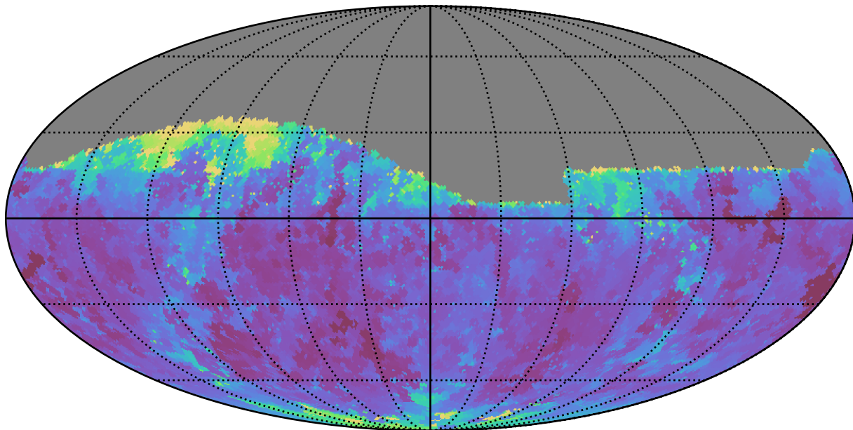
weather_cloudso30v3.4_10yrs Yr 1 z band: Min seeingGeom
