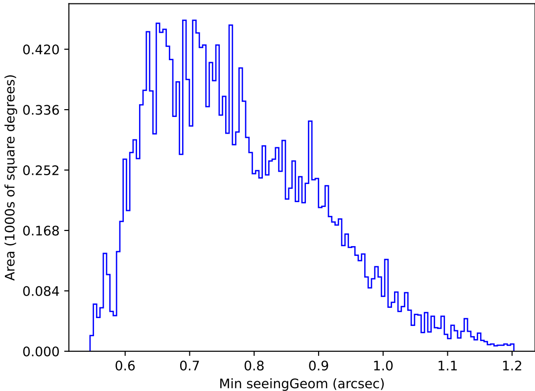
weather_cloudso30v3.4_10yrs Yr 1 u band: Min seeingGeom
