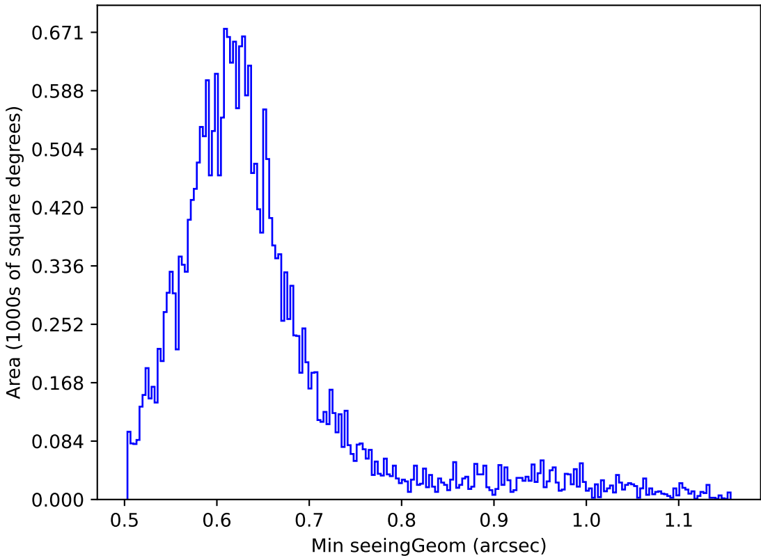
weather_cloudso30v3.4_10yrs Yr 1 r band: Min seeingGeom
