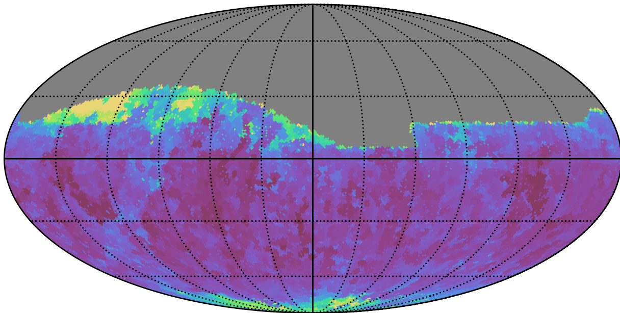
weather_cloudso30v3.4_10yrs Yr 1 i band: Min seeingGeom
