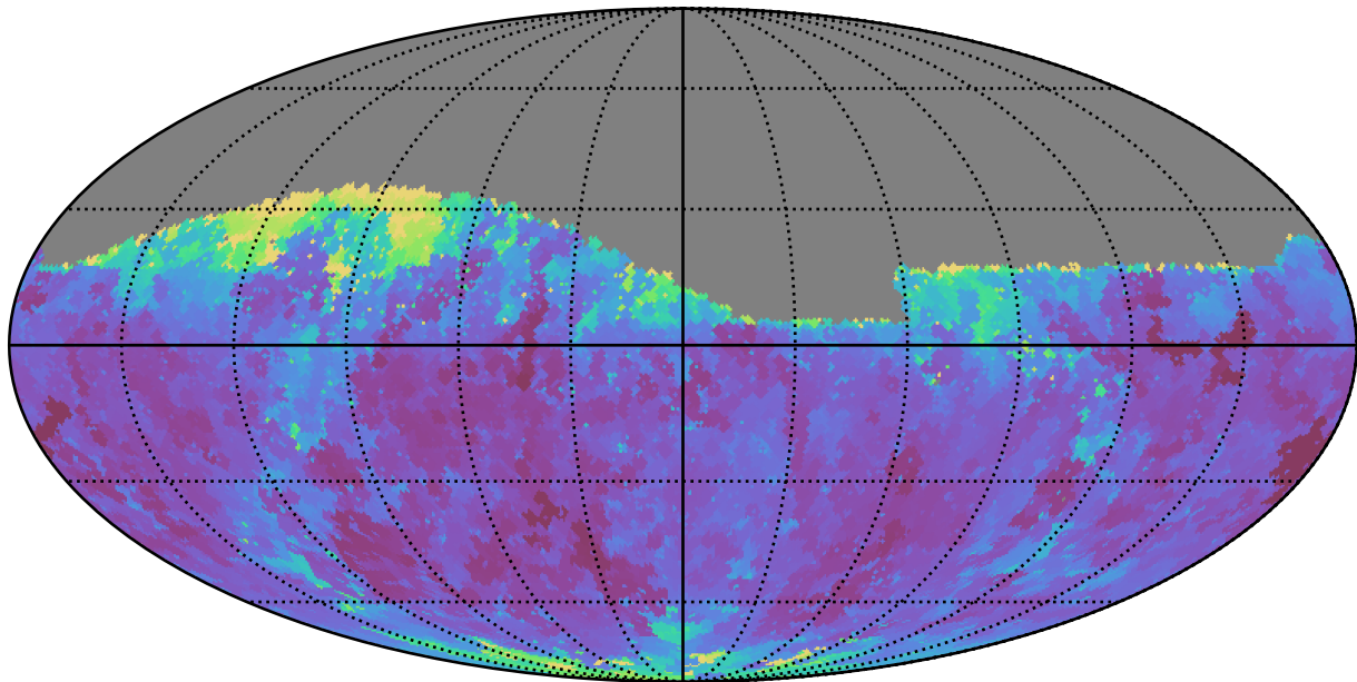
weather_cloudso30v3.4_10yrs Yr 1 z band: Min seeingEff
