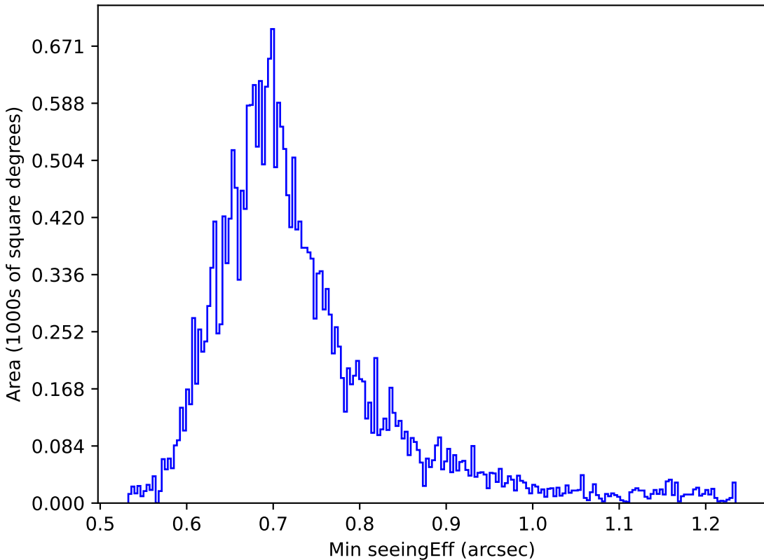
weather_cloudso30v3.4_10yrs Yr 1 z band: Min seeingEff
