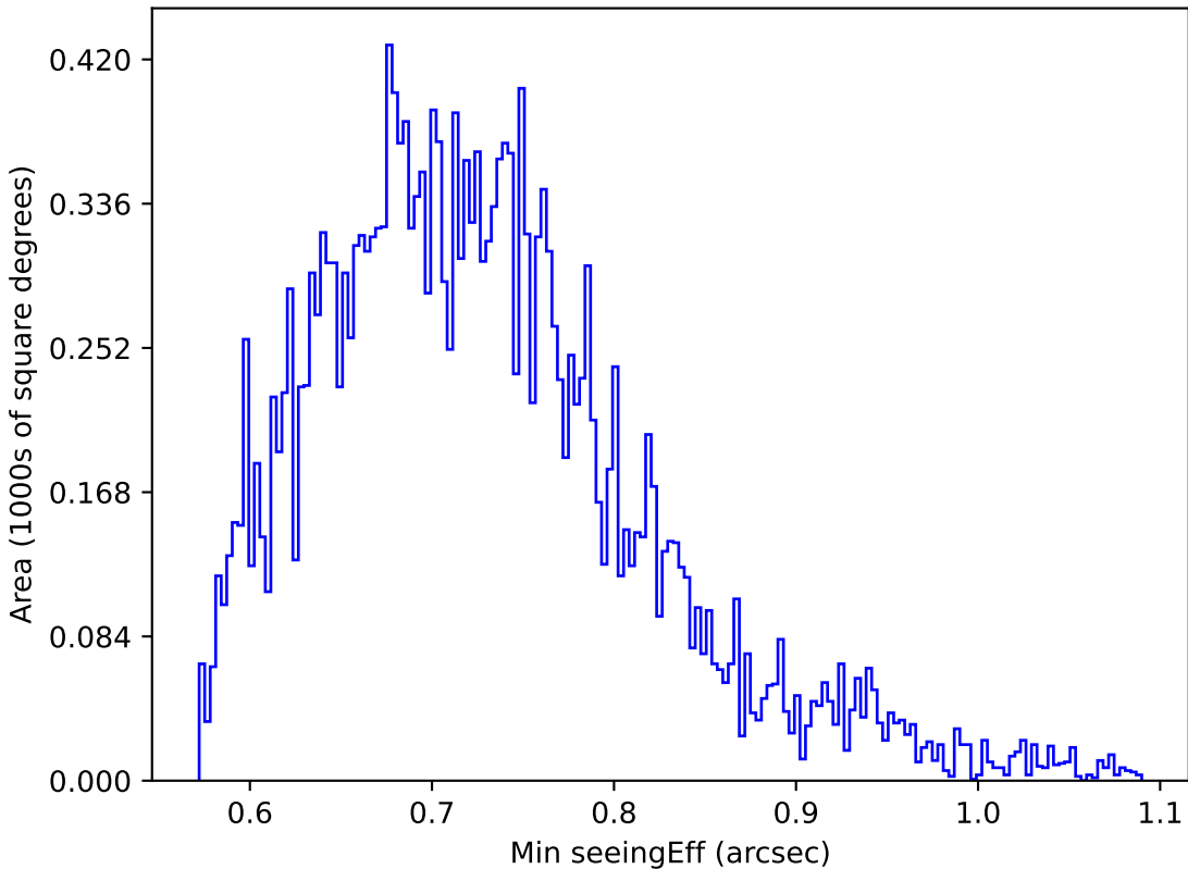
weather_cloudso30v3.4_10yrs Yr 1 y band: Min seeingEff
