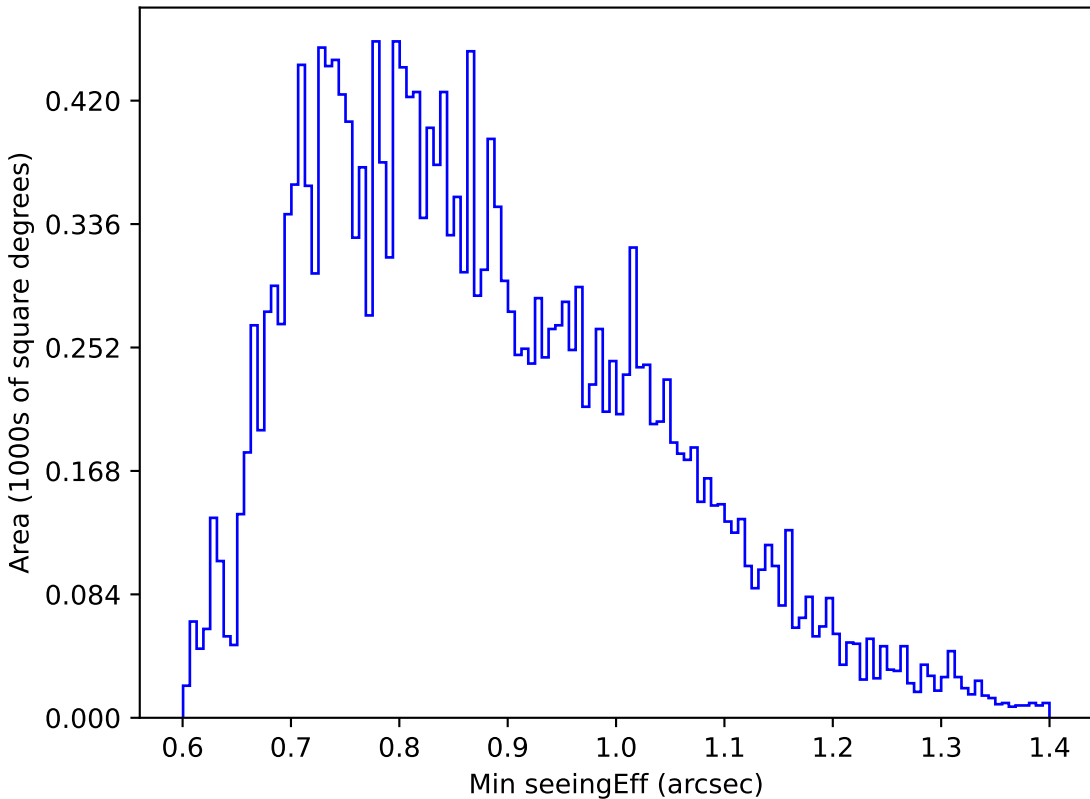
weather_cloudso30v3.4_10yrs Yr 1 u band: Min seeingEff
