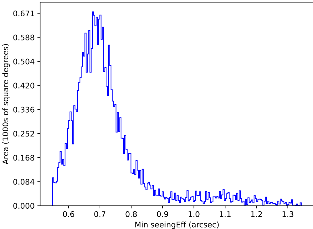
weather_cloudso30v3.4_10yrs Yr 1 r band: Min seeingEff
