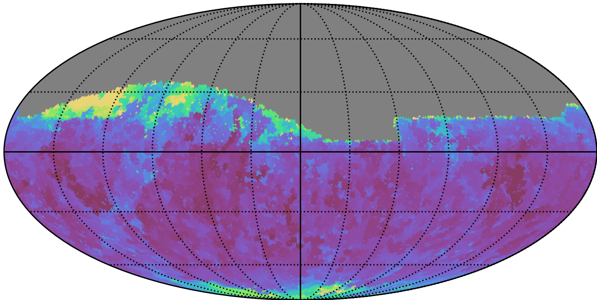
weather_cloudso30v3.4_10yrs Yr 1 i band: Min seeingEff
