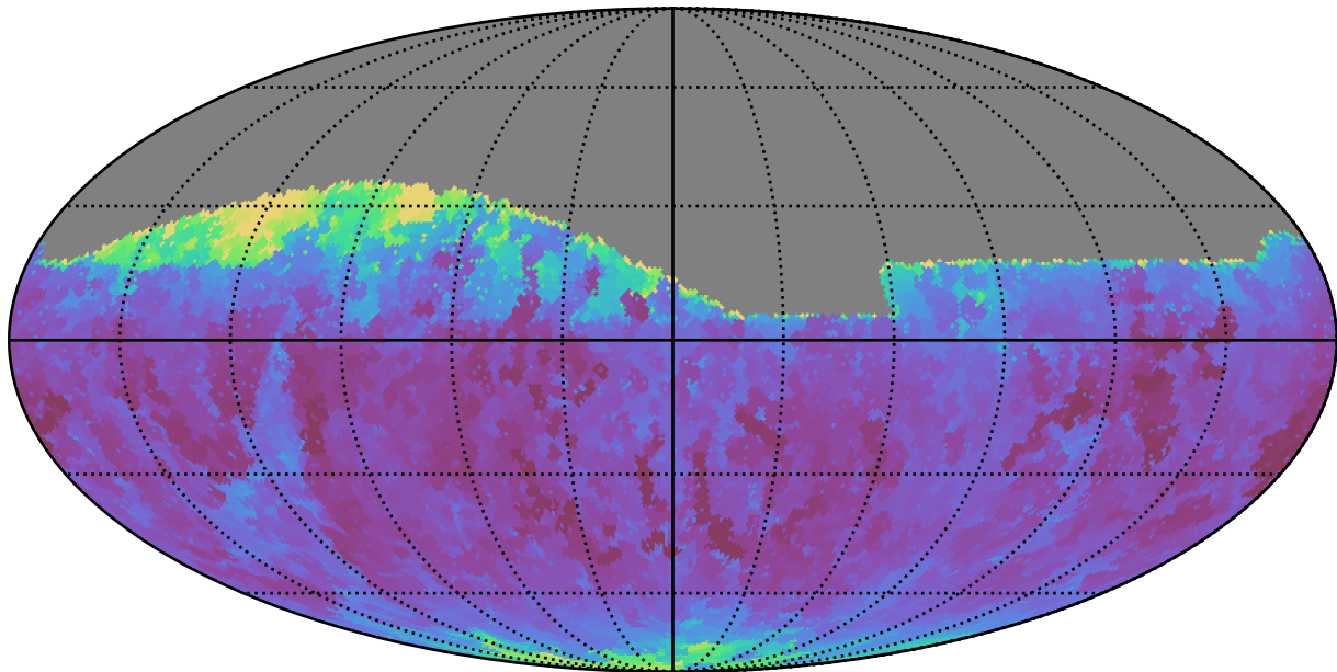
weather_cloudso30v3.4_10yrs Yr 1 all bands: Min seeingEff
