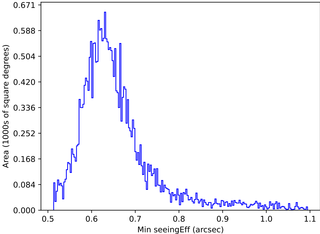
weather_cloudso30v3.4_10yrs Yr 1 all bands: Min seeingEff
