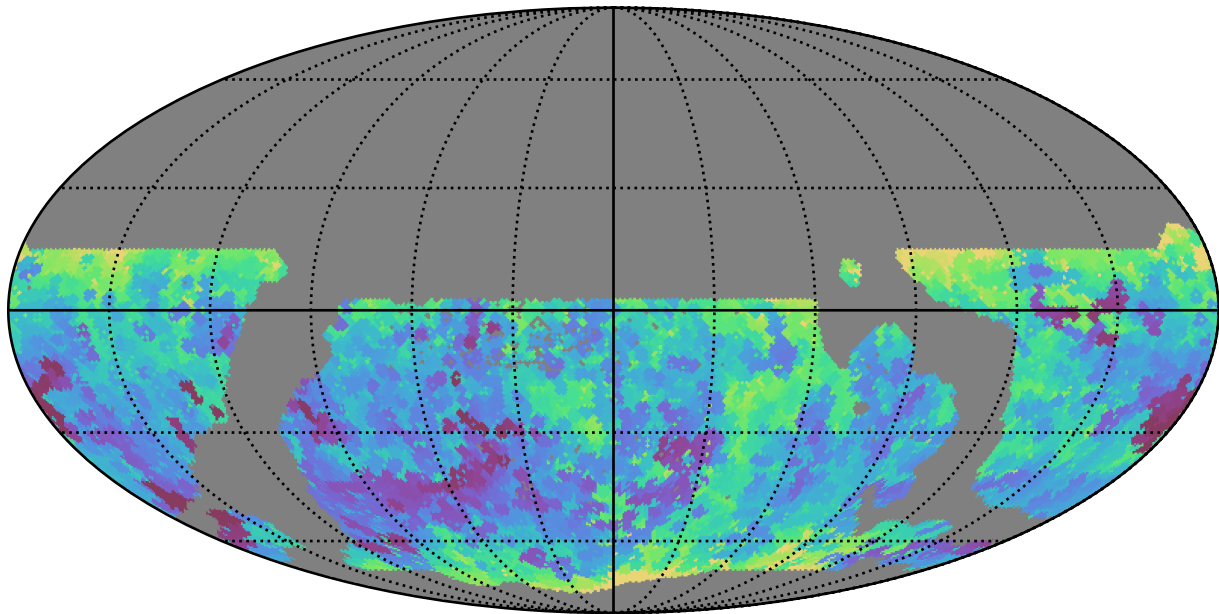
weather_cloudso30v3.4_10yrs WFD z band: Min seeingEff
