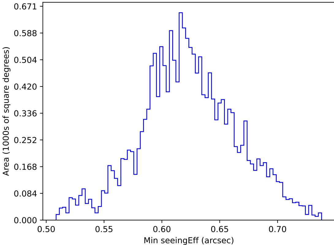
weather_cloudso30v3.4_10yrs WFD z band: Min seeingEff
