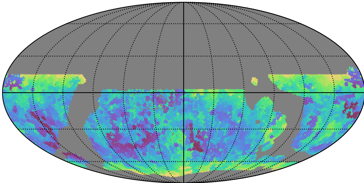
weather_cloudso30v3.4_10yrs WFD y band: Min seeingEff
