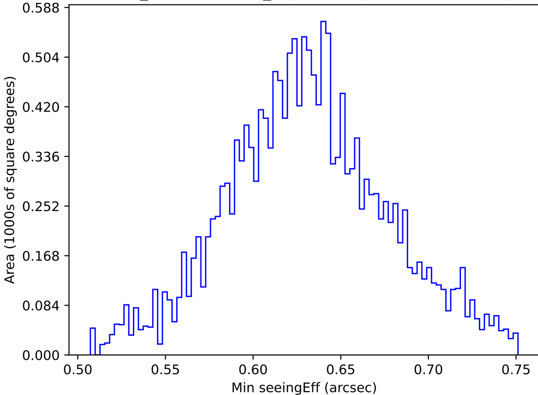
weather_cloudso30v3.4_10yrs WFD y band: Min seeingEff
