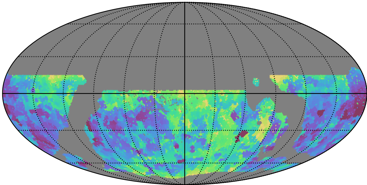
weather_cloudso30v3.4_10yrs WFD u band: Min seeingEff
