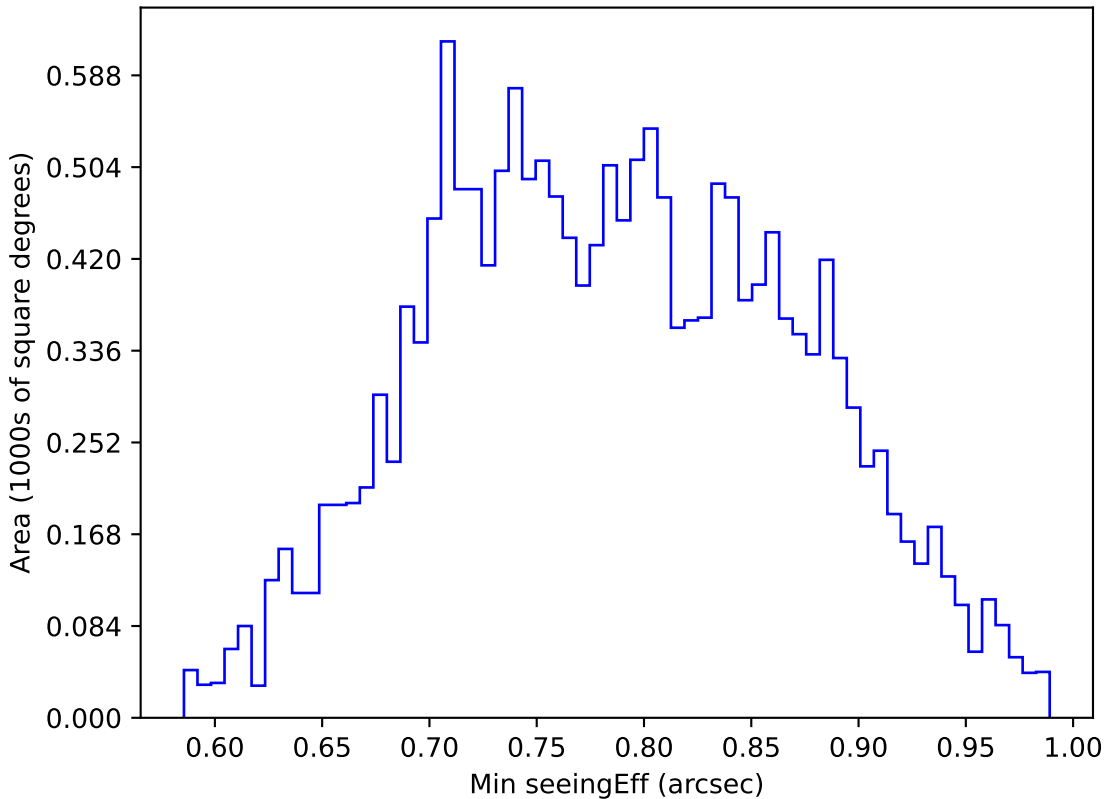
weather_cloudso30v3.4_10yrs WFD u band: Min seeingEff
