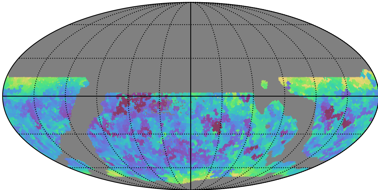
weather_cloudso30v3.4_10yrs WFD r band: Min seeingEff
