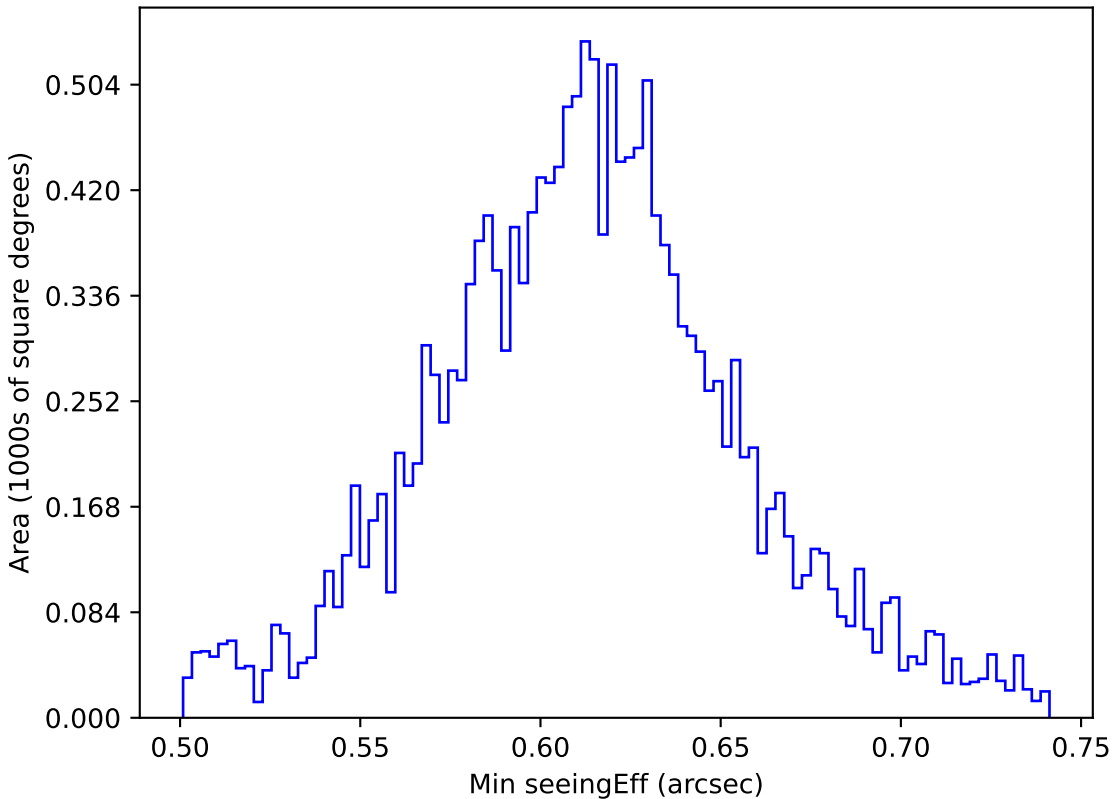
weather_cloudso30v3.4_10yrs WFD r band: Min seeingEff
