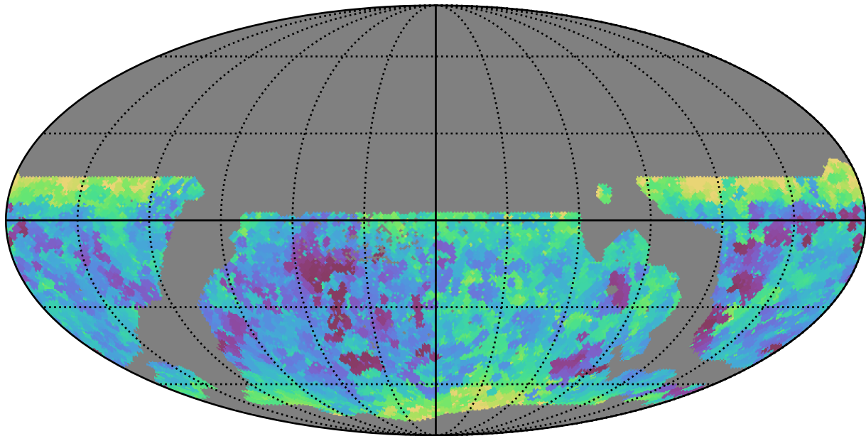
weather_cloudso30v3.4_10yrs WFD i band: Min seeingEff
