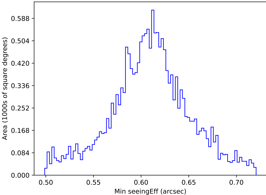
weather_cloudso30v3.4_10yrs WFD i band: Min seeingEff
