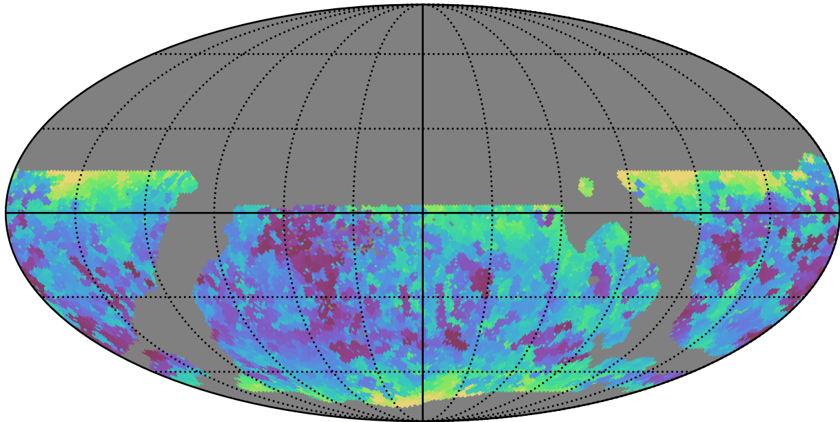
weather_cloudso30v3.4_10yrs WFD all bands: Min seeingEff
