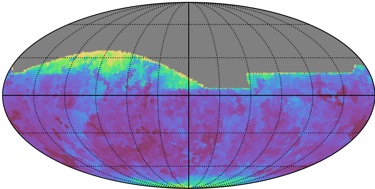
weather_cloudso30v3.4_10yrs All sky z band: Min seeingEff
