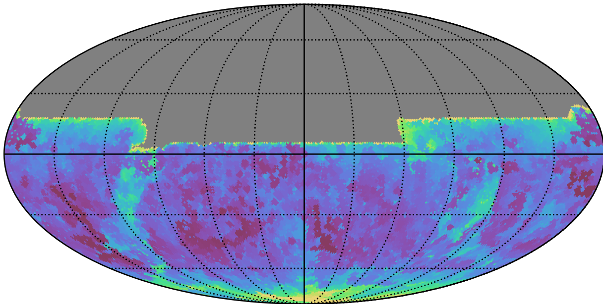
weather_cloudso30v3.4_10yrs All sky y band: Min seeingEff
