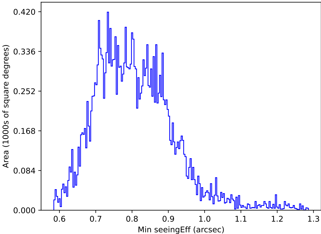
weather_cloudso30v3.4_10yrs All sky u band: Min seeingEff
