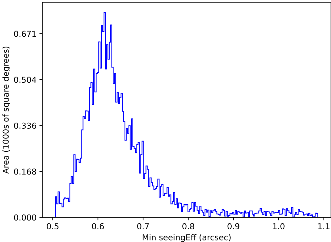
weather_cloudso30v3.4_10yrs All sky r band: Min seeingEff
