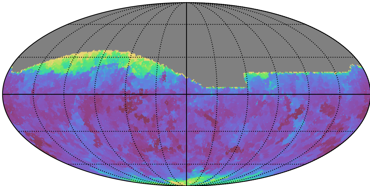
weather_cloudso30v3.4_10yrs All sky g band: Min seeingEff
