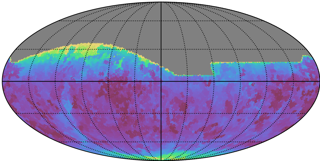
weather_cloudso30v3.4_10yrs All sky all bands: Min seeingEff
