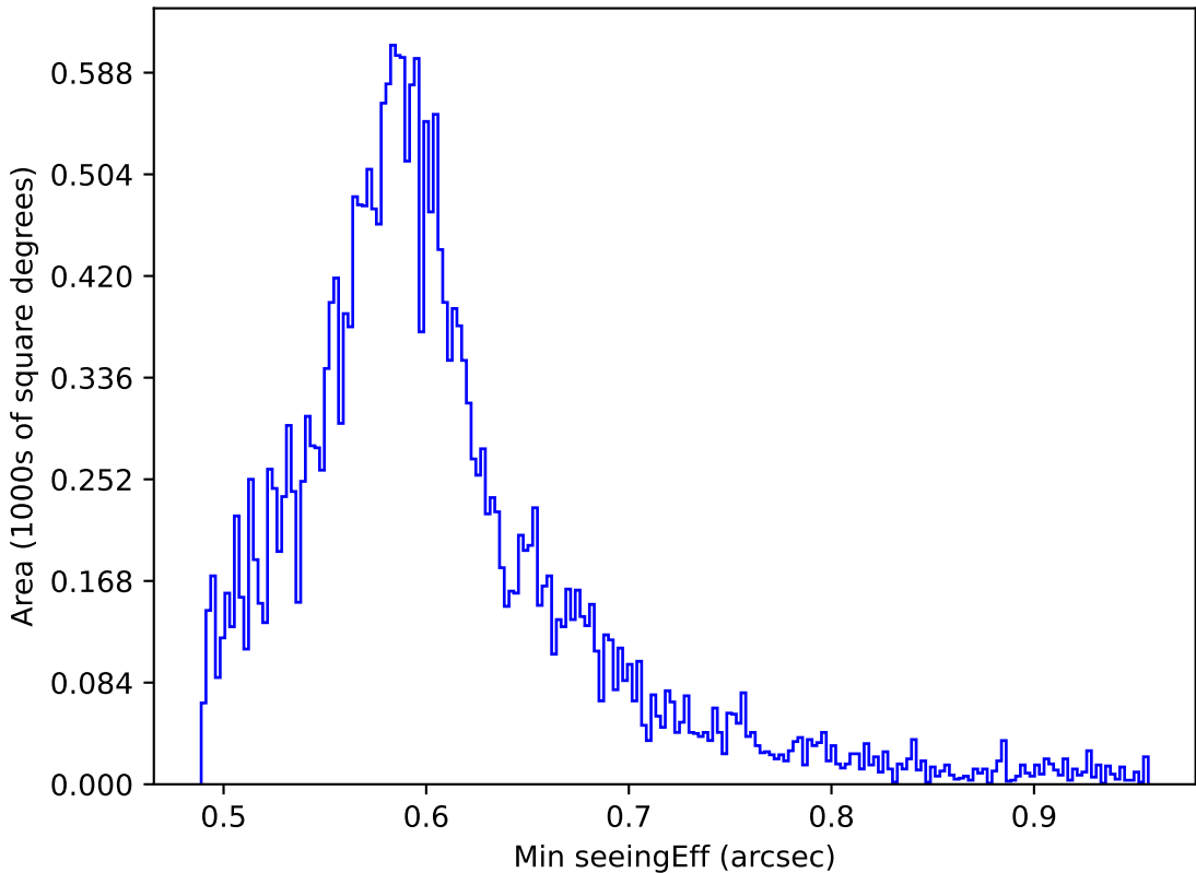
weather_cloudso30v3.4_10yrs All sky all bands: Min seeingEff
