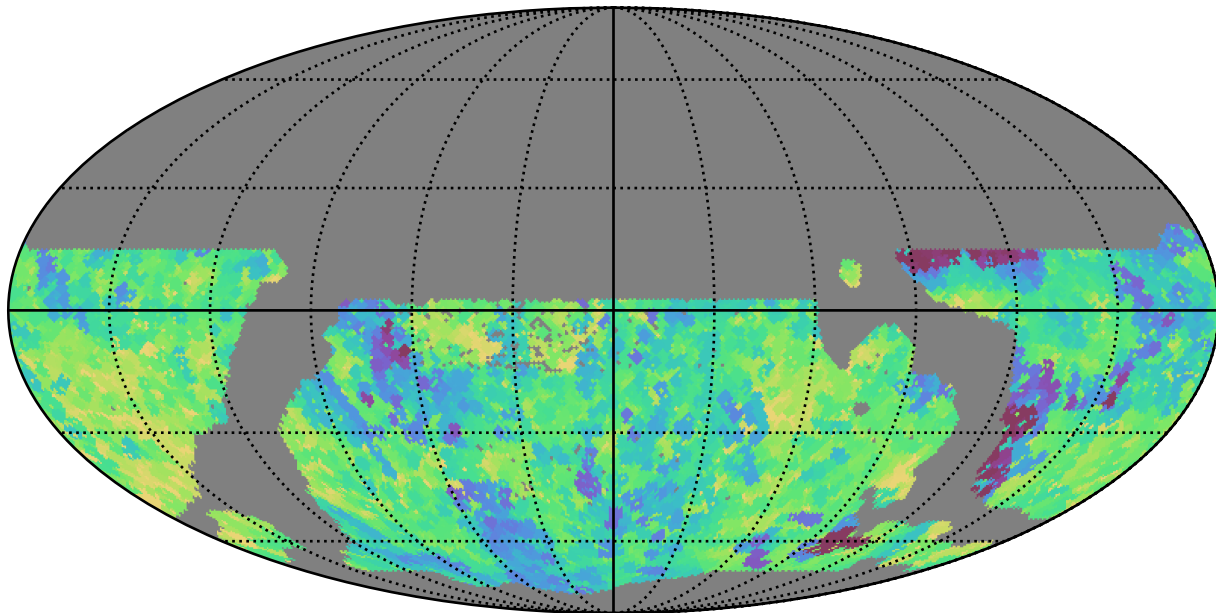
weather_cloudso30v3.4_10yrs WFD all bands: Min saturation_mag
