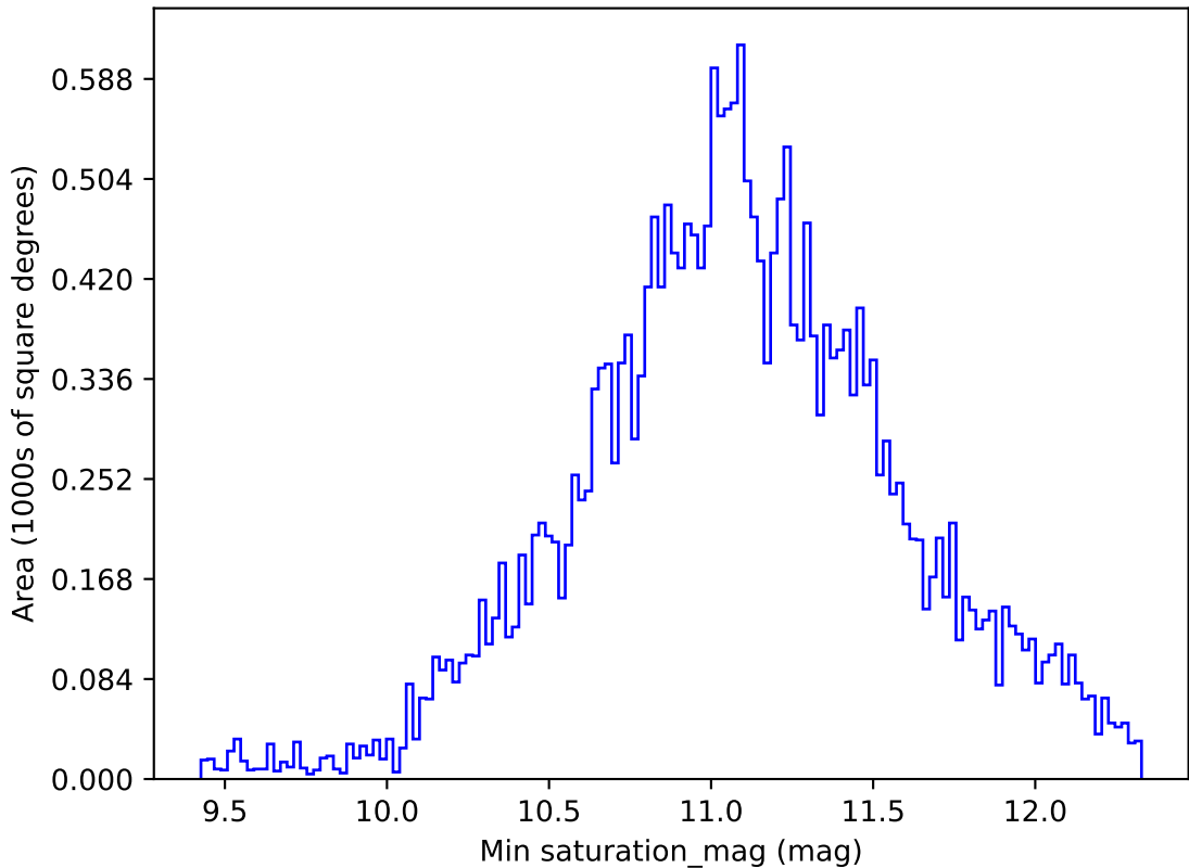
weather_cloudso30v3.4_10yrs All sky all bands: Min saturation_mag
